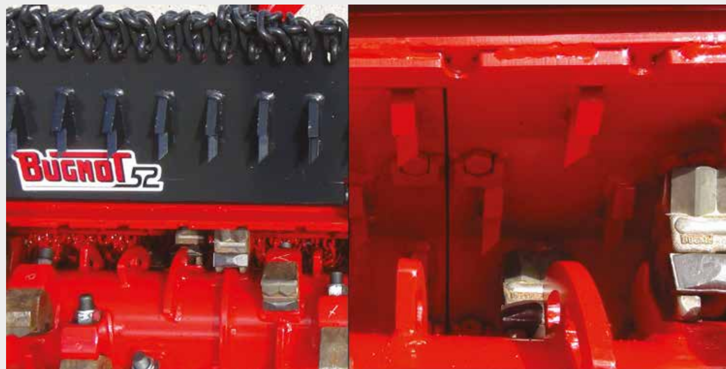
For an optimum grinding, the mulcher is fitted with counter knife shearbars at the front and above the rotor as well as on the hydraulically operated rear door
